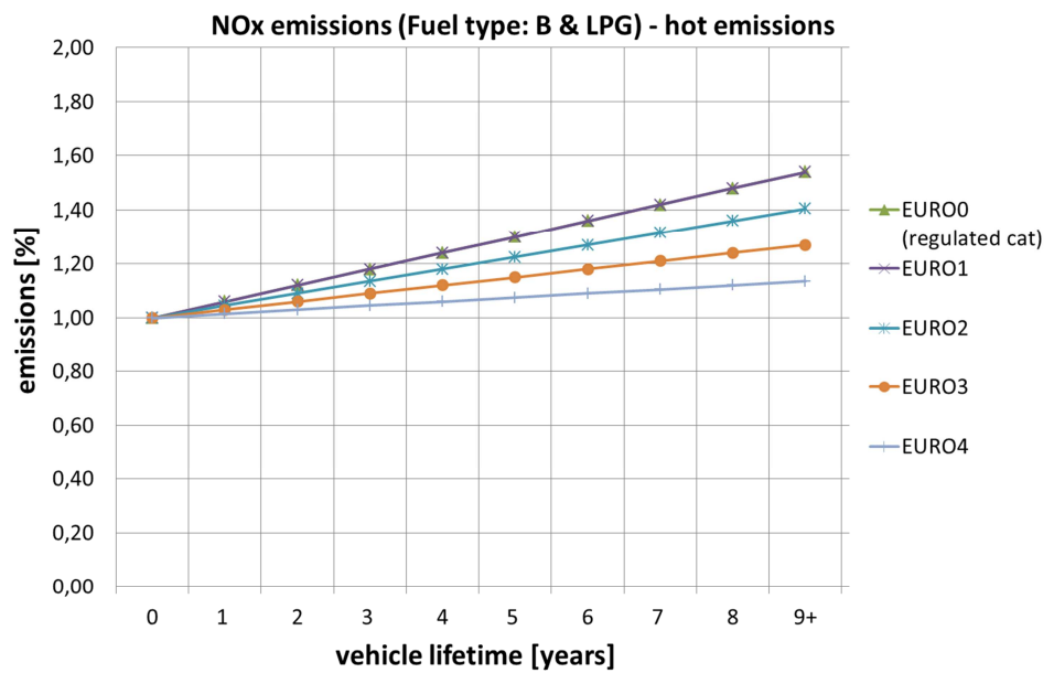
Figure 6 NOx deterioration factors for hot emissions, petrol vehicle (1=100%).
