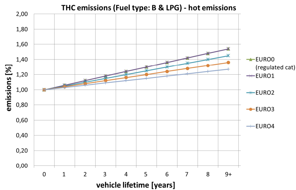
Figure 4 THC deterioration factors for hot emissions, petrol vehicle (1=100%).
