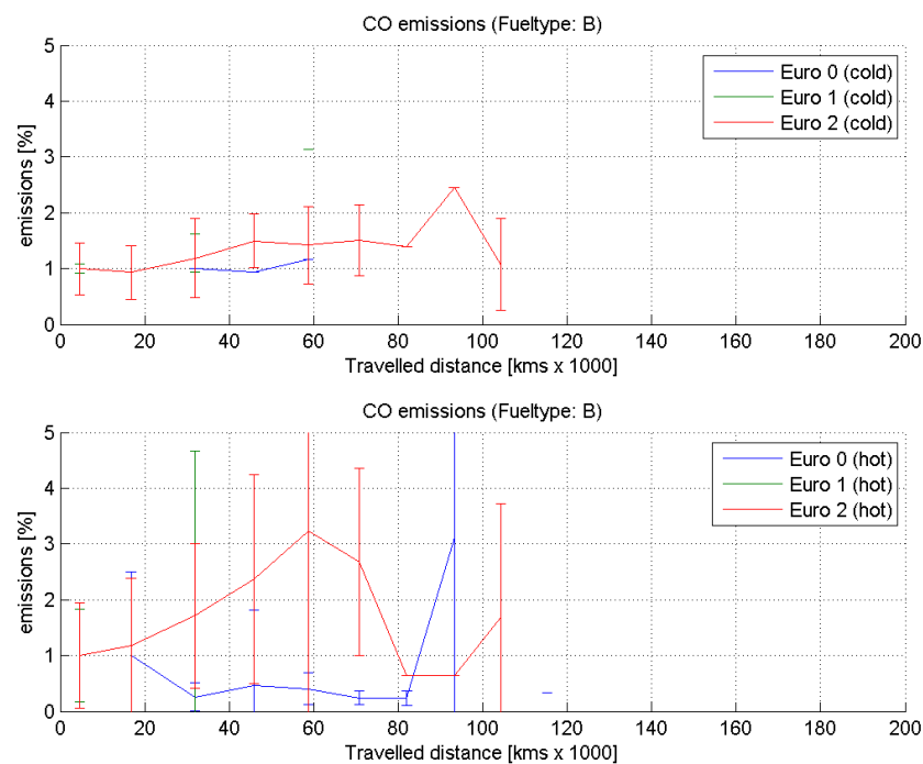
Figure 10 CO results of petrol vehicles as a function of the vehicle distance travelled (1=100%).
