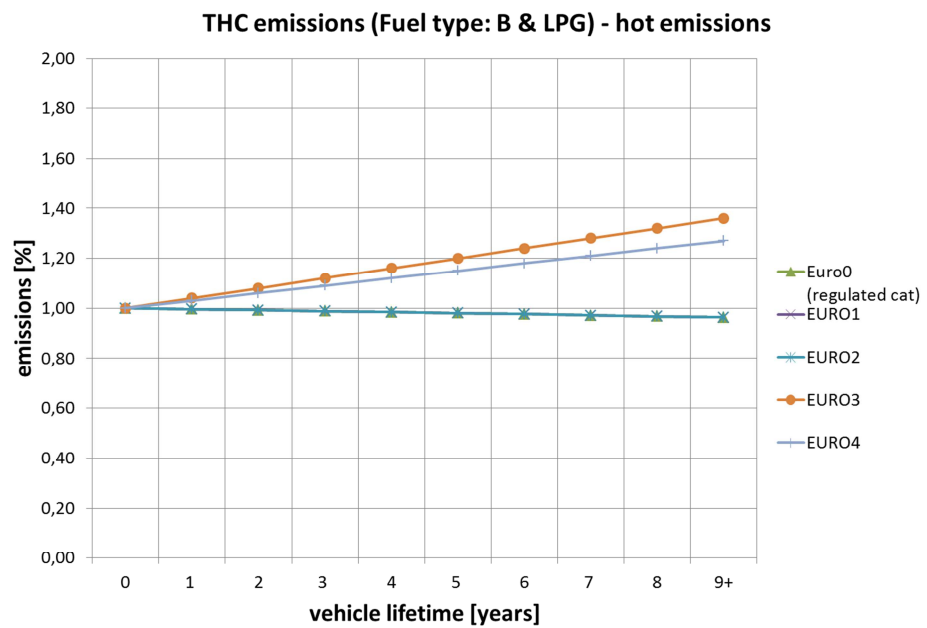
Figure 20 THC deterioration factors based on hot emission measurements, petrol vehicle (1=100%).
