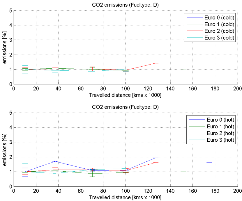
Figure 15 CO 2 test results of diesel vehicles as a function of the vehicle distance travelled (1=100%).
