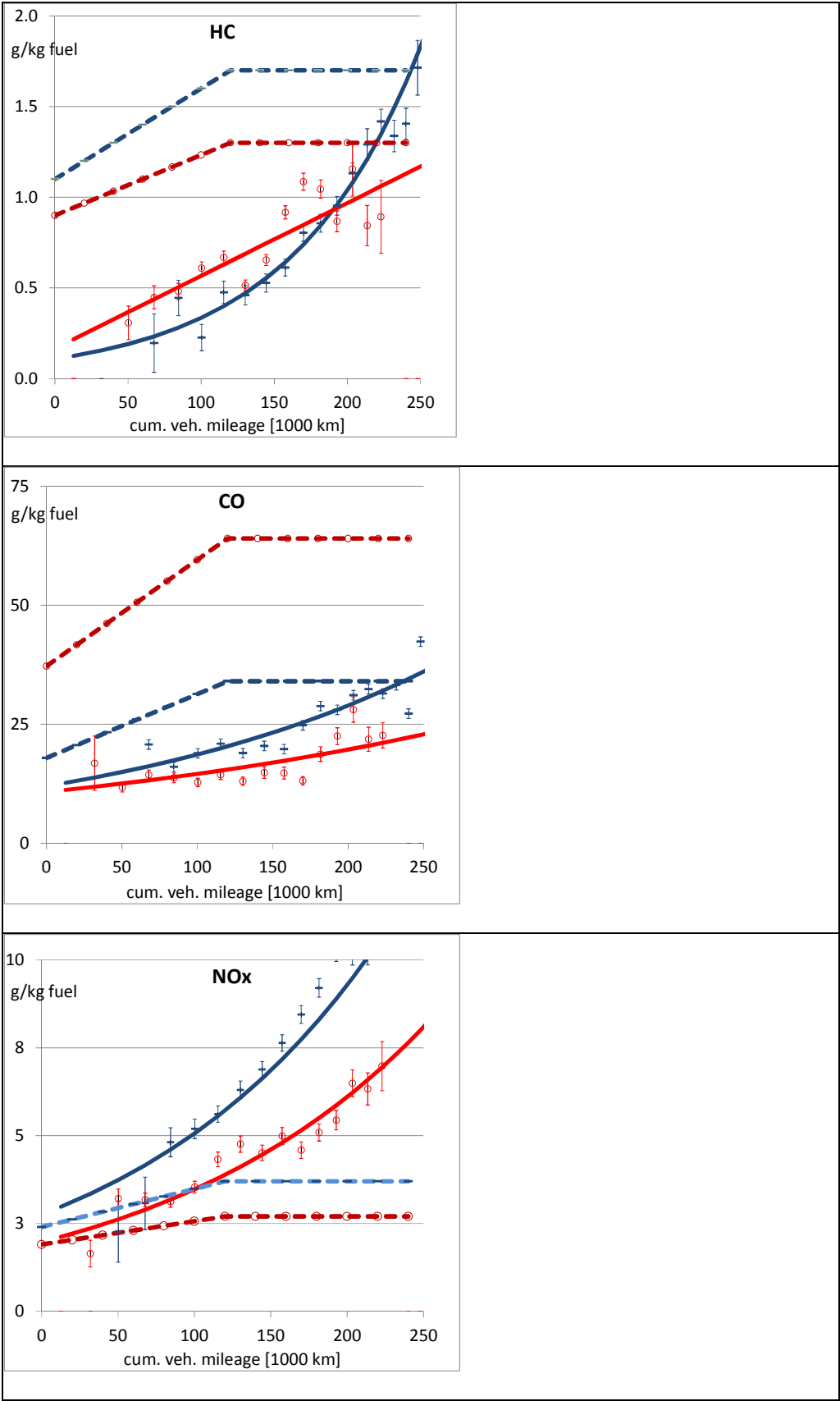
Figure 23 Petrol hot emissions [IIASA, 2014] (the solid lines) in comparison with current TNO emission factors (dashed lines), Euro 1 (blue), Euro 2 (red).
