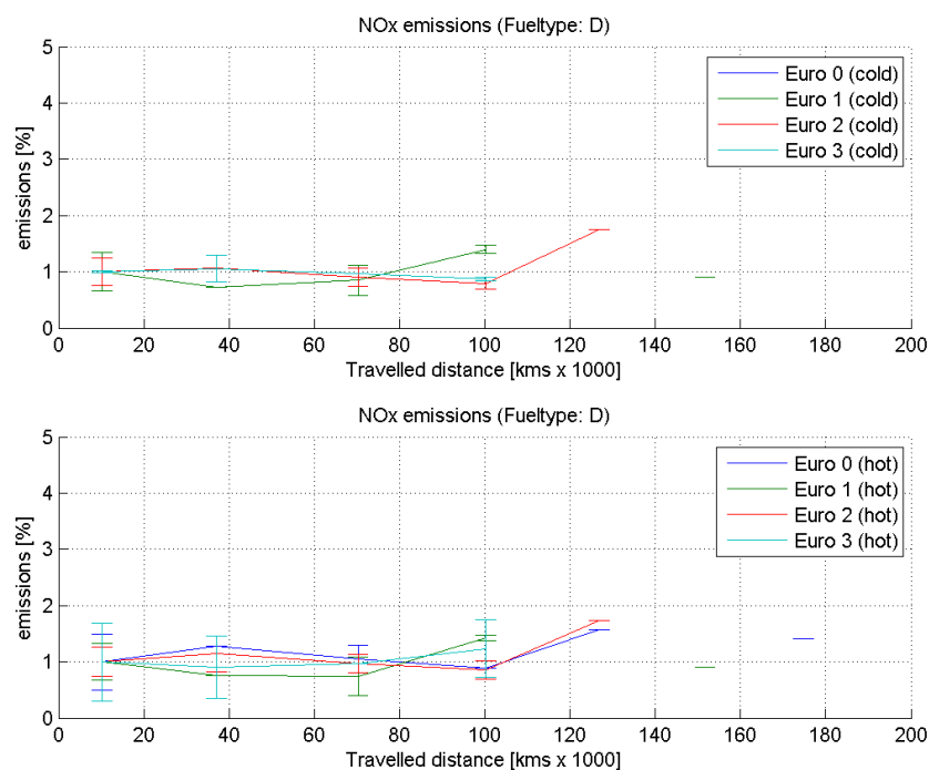
Figure 16 NO x test results of diesel vehicles as a function of the vehicle distance travelled (1=100%).
