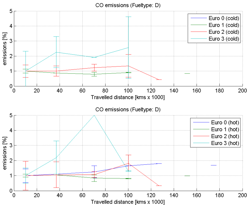
Figure 14 CO test results of diesel vehicles as a function of the vehicle distance travelled (1=100%).
