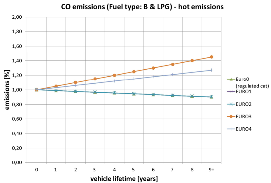
Figure 18 CO deterioration factors based on hot emission measurements, petrol vehicle (1=100%).
