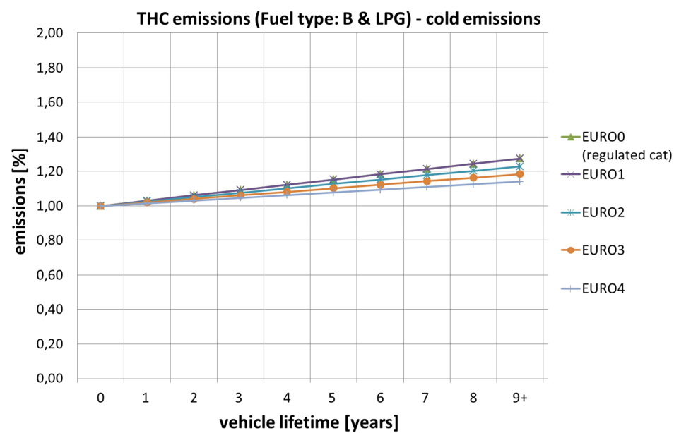
Figure 3 THC deterioration factors for cold start emissions, petrol vehicle (1=100%).
