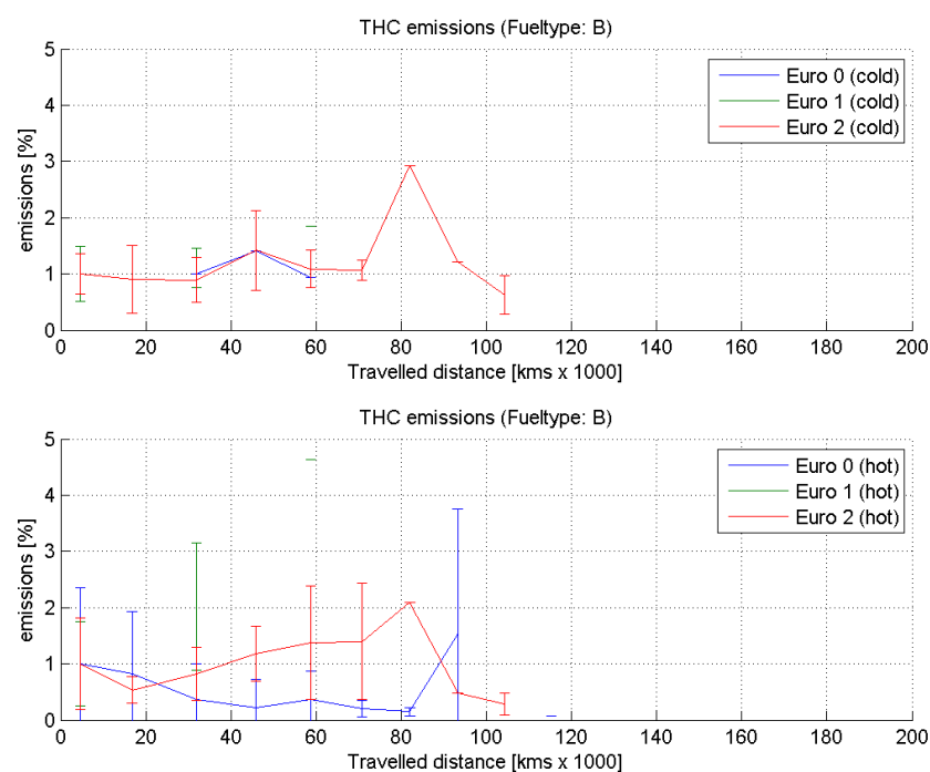
Figure 9 THC results of petrol vehicles as a function of the vehicle distance travelled (1=100%).
