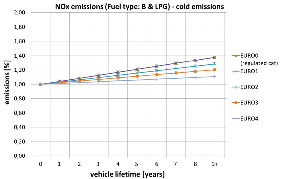
Figure 5 NOx deterioration factors for cold start emissions, petrol vehicle (1=100%).
