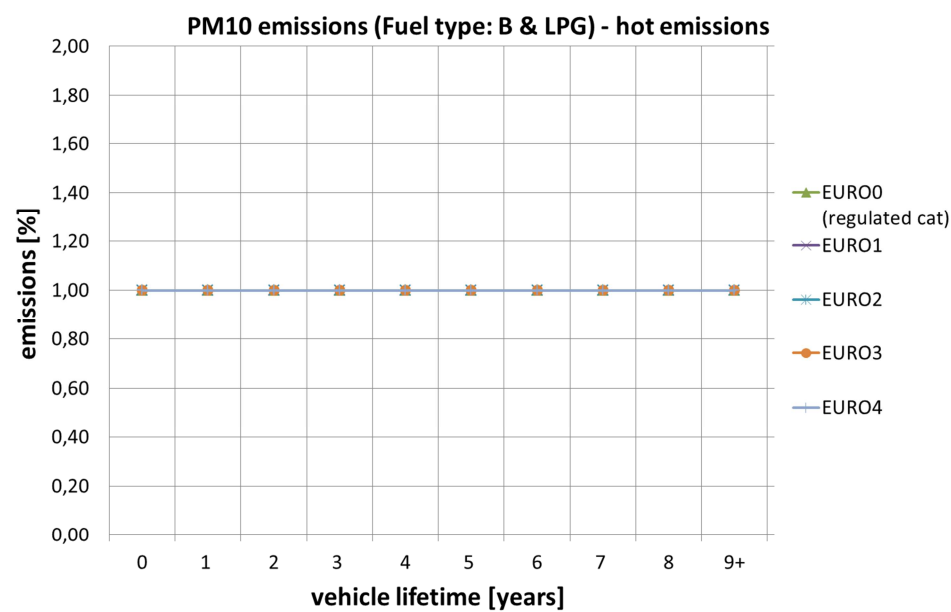
Figure 8 PM10 deterioration factors for hot emissions, petrol vehicle (1=100%).
