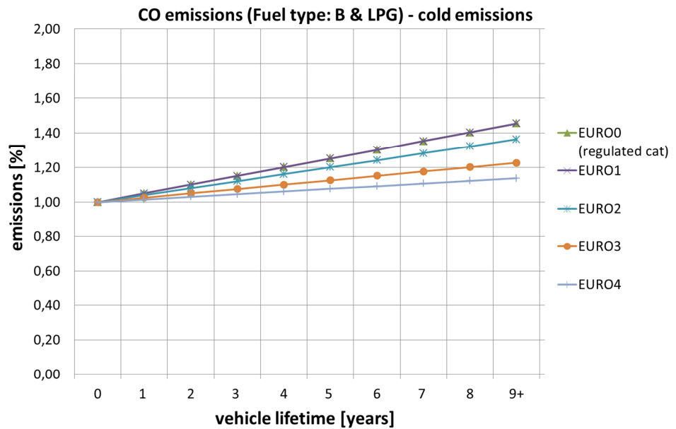
Figure 1 CO deterioration factors for cold start emissions, petrol vehicle (1=100%) (markers do not indicate measuring points).
