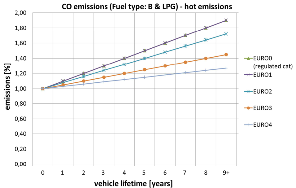
Figure 2 CO deterioration factors for hot MVEG cycle emissions, petrol vehicle (1=100%) B = Petrol.
