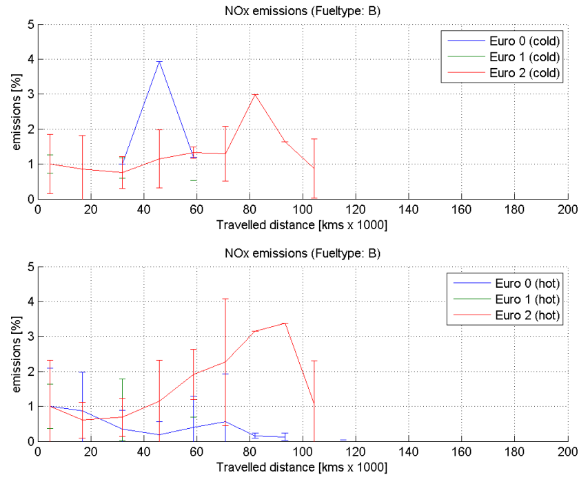
Figure 12 NO x test results of petrol vehicles as a function of the vehicle distance travelled (1=100%).
