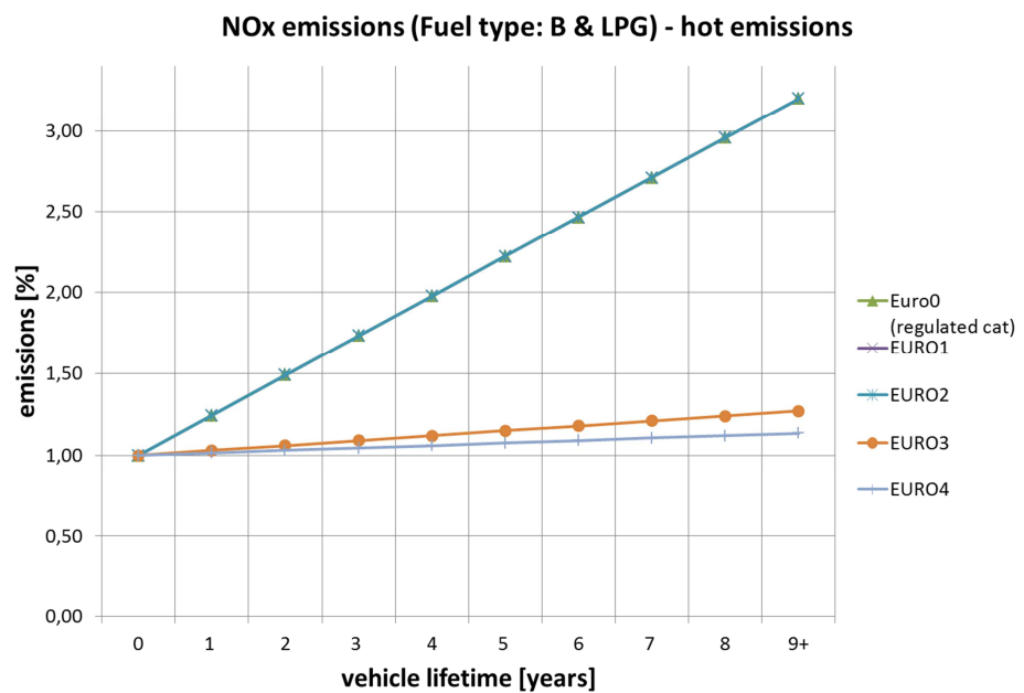
Figure 22 NOx deterioration factors based on hot emission measurements, petrol vehicle (1=100%).
