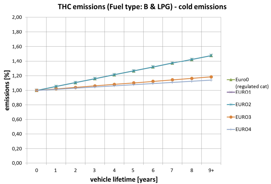
Figure 19 THC deterioration factors based cold emission measurements, petrol vehicle (1=100%).
