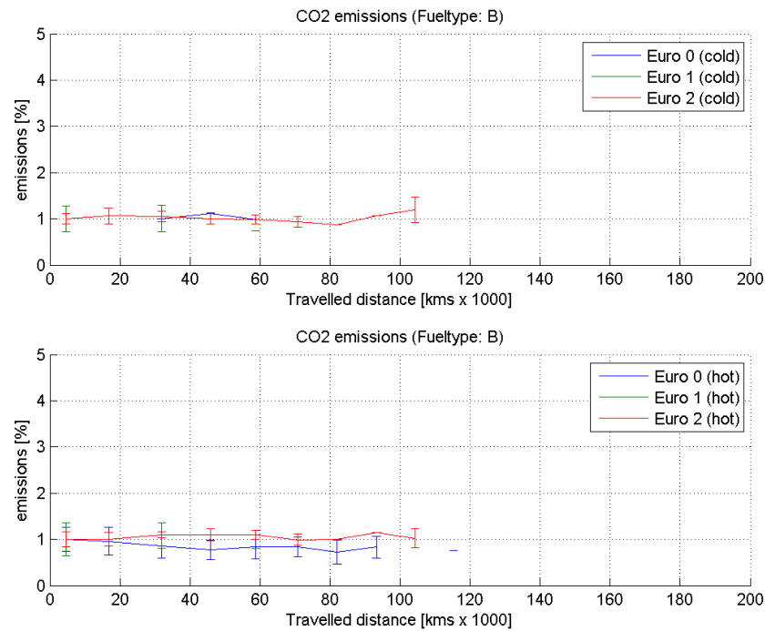
Figure 11 CO 2 test results of petrol vehicles as a function of the vehicle distance travelled (1=100%).
