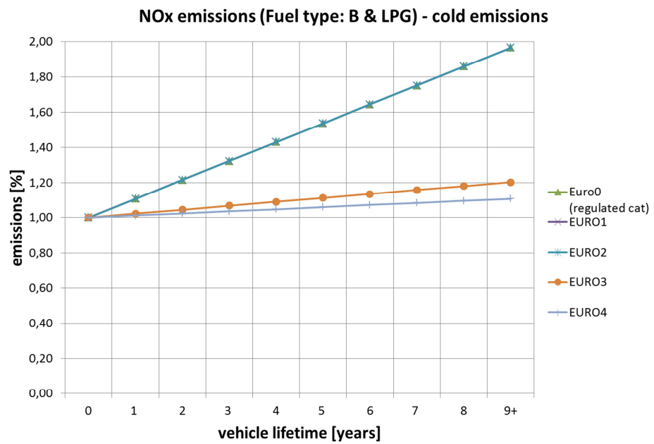
Figure 21 NOx deterioration factors based on cold emission measurements, petrol vehicle (1=100%).
