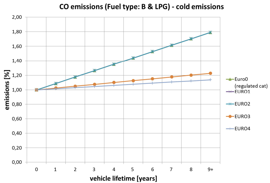
Figure 17 CO deterioration factors based on cold emission measurements, petrol vehicle (1=100%).
